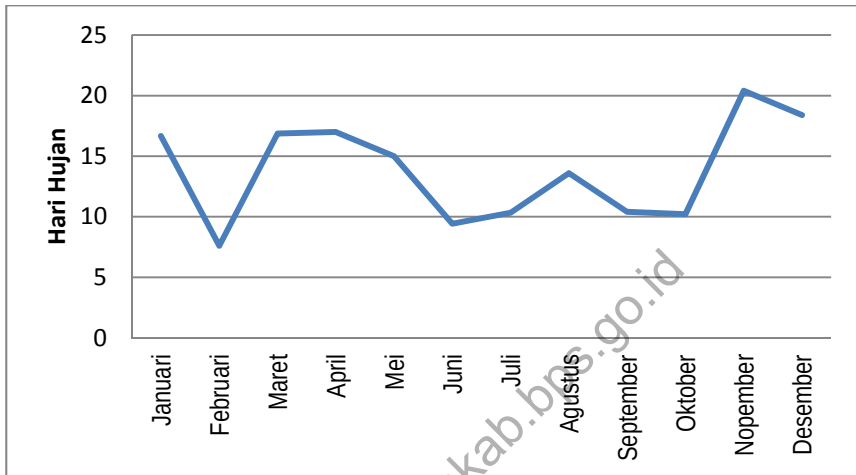
Grafik : 1.1. Rata-rata Hari Hujan menurut Bulan 2015 Graphic Average of Rainy Days by Month 2015
